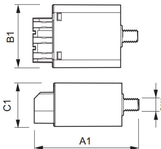
Amorceur SKD 578-S IM-SHP 35-600w 220-240V 50/60Hz PHILIPS
