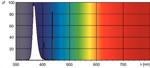
XDPO_XUAPLS_10_110_210-Spectral power distribution Colour
